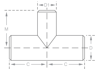
Reducer Tee
