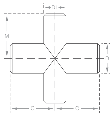
Reducer Cross
