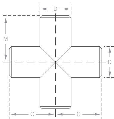
Cross Tee
