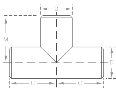
Equal Tee
