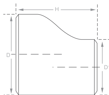
Eccentric Reducer
