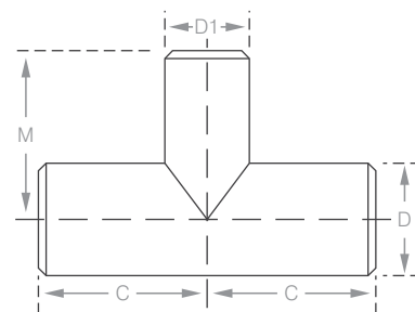
Reducer Tee
