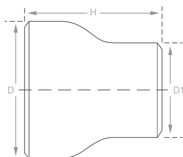
Concentric Reducer
