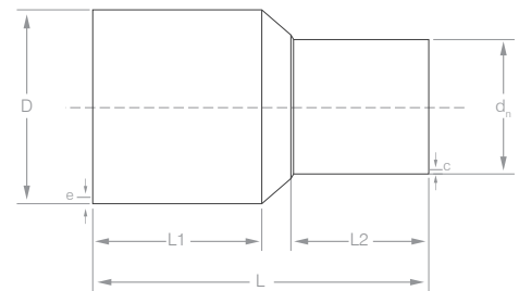
Concentric Reducer
