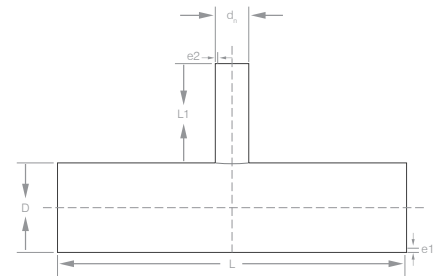
Reducer Tee
