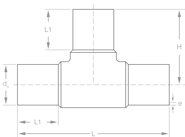
Equal Tee
