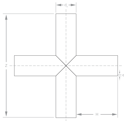
Cross Tee
