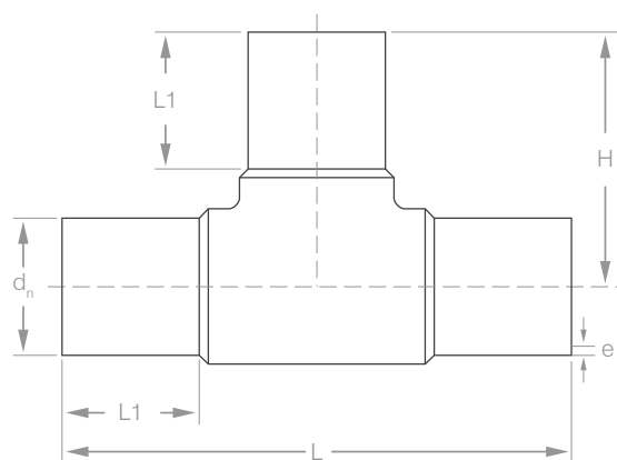
Equal Tee
