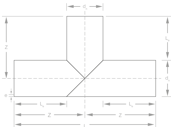
Equal Tee
