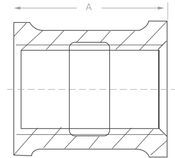
Straight Coupling
