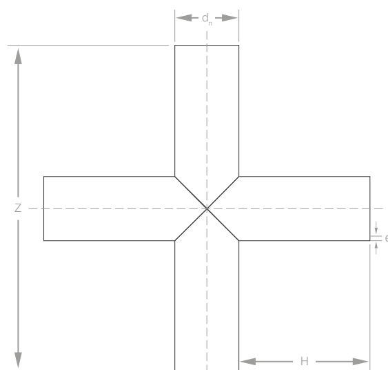
Cross Tee
