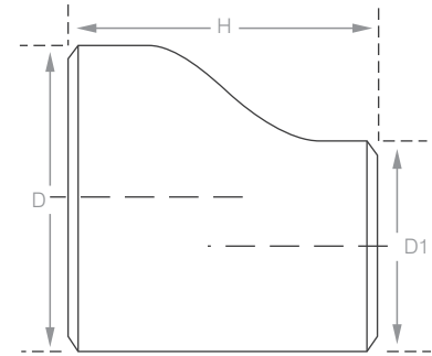
Eccentric Reducer
